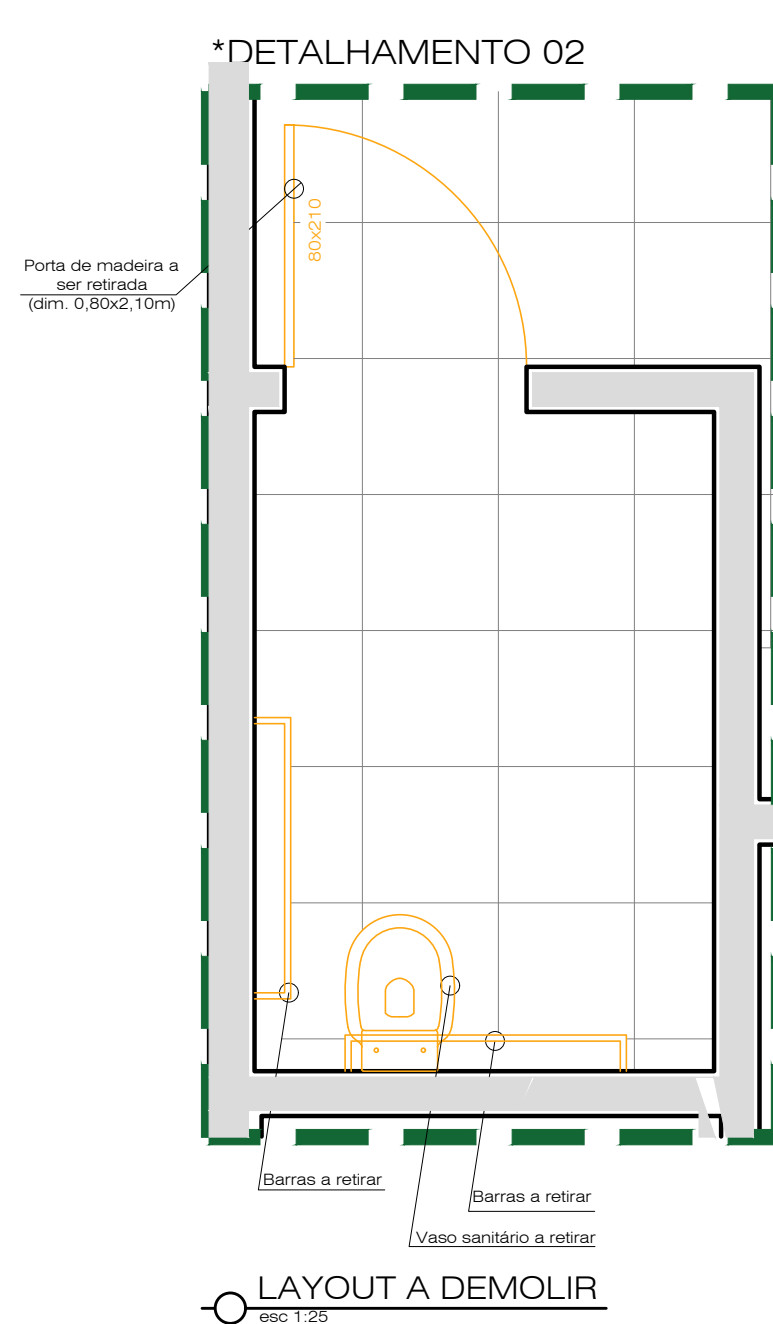
LAYOUT A DEMOLIR
