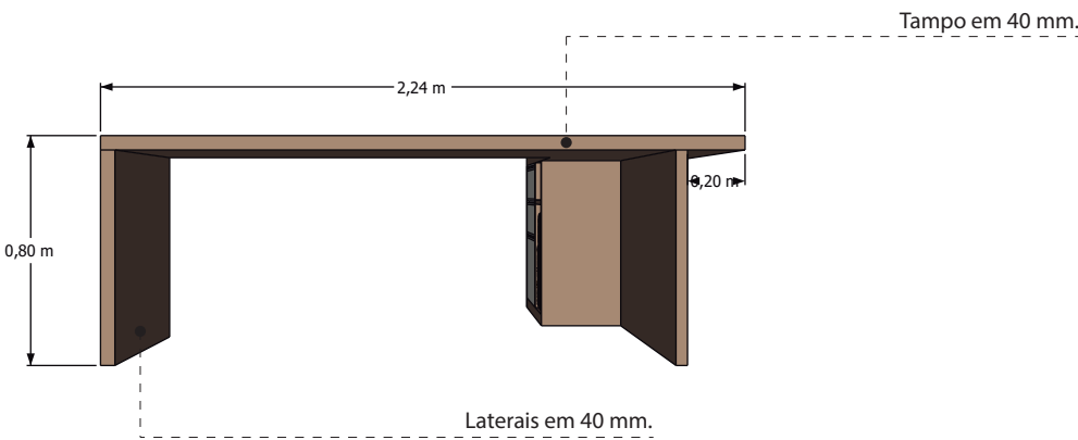
Vista Frontal
